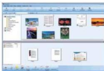
Ventana Sharpdesk
